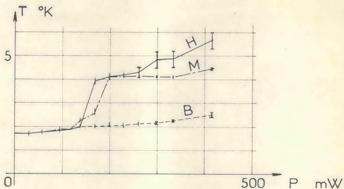
FIG.9 : Superfluid helium T = 1.7 \text{ K} ; p = 1 \text{ atm}
