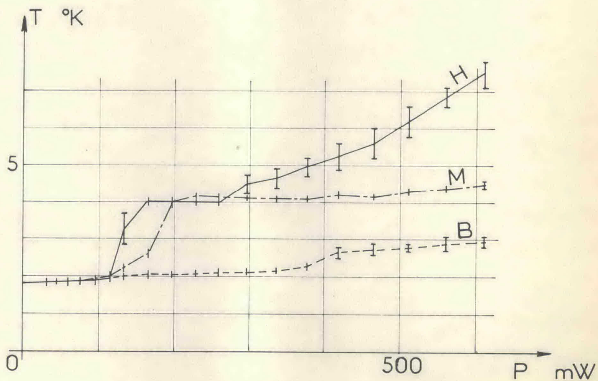
FIG.10 : Superfluid helium T = 1.8 \text{ K} ; p = 1 \text{ atm}
